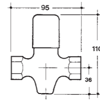
NC2729 Stopcock
