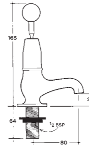
NC2754 Bibcock
