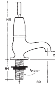
NC2750B Pillar Valve
