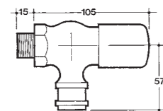
NC2726 Bibcock
