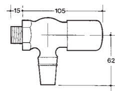
NC2726 Bibcock
