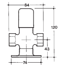
NC2729 Stopcock
