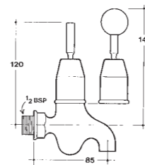
NC2754 Bibcock
