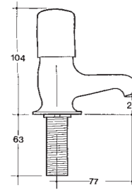
NC2720 Pillar Valve
