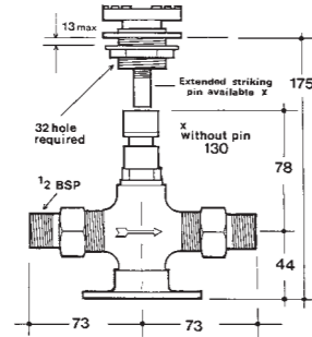
NC2728 Stopcock
